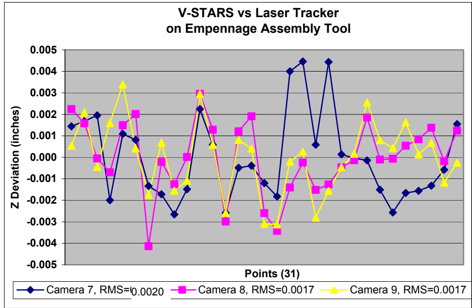
Figure 6c –Z Deviations V-STARS Vs. Laser Tracker Results for Empennage Assembly Tool
