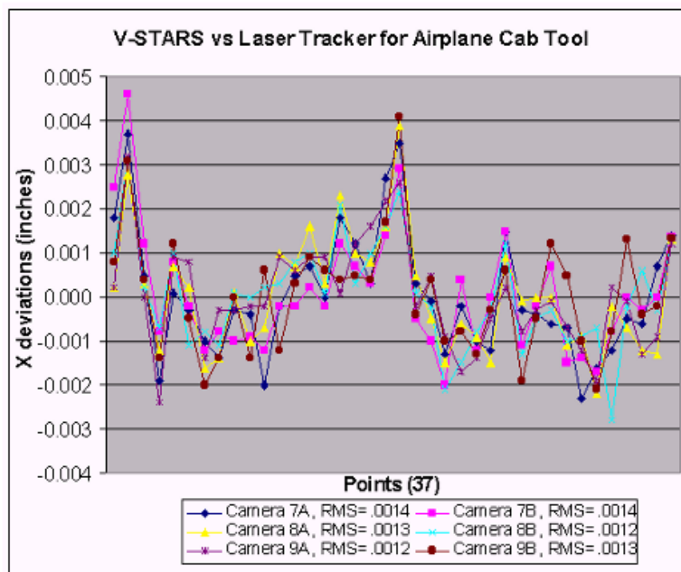
Figure 3a –X Deviations V-STARS Vs Laser Tracker Results for Airplane Cab Tool
