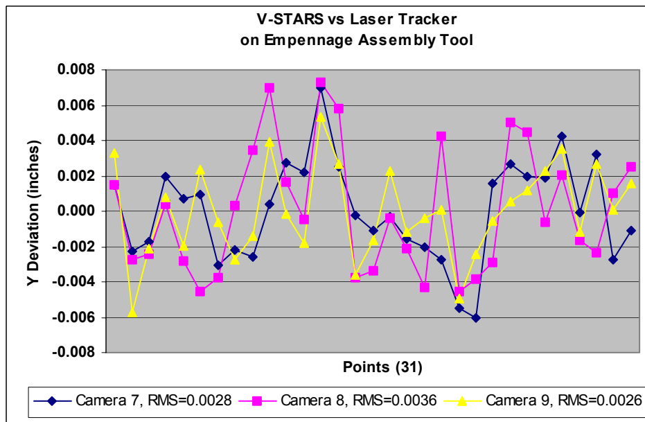
Figure 6b –Y Deviations V-STARS Vs Laser Tracker Results for Empennage Assembly Tool
