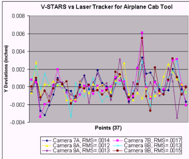
Figure 3b –Y Deviations V-STARS Vs Laser Tracker Results for Airplane Cab Tool
